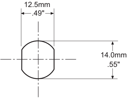
Receptacle - Pinout (front view)
